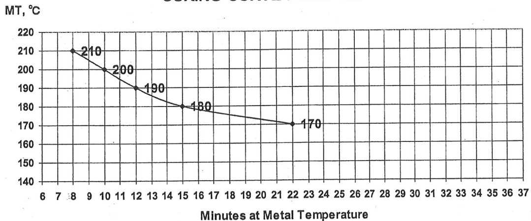
PPG ENVIROCRON - RECOMMENDED BAKE CURING CURVE PCMC-003
